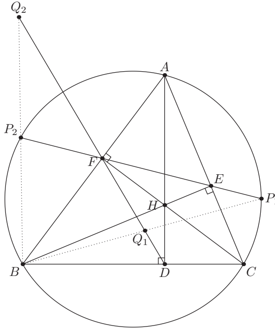
Figure 1.7A. IMO Shortlist 2010, Problem G1 (Example 1.35).
