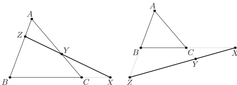
Figure 3.3A. The two cases of Menelaus's theorem.
